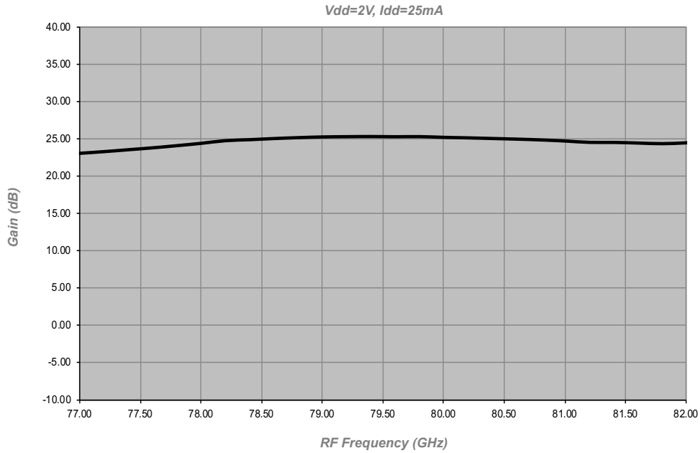
Figure 1 Gain
