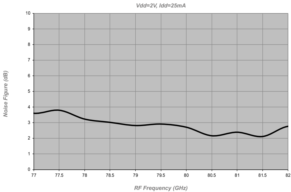
Figure 2 Noise Figure
